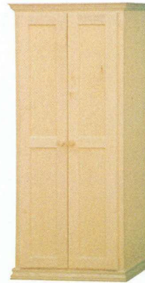
CA_3030 Storage Cabinet 25" w x 58" h x 13" d 4 adjustable shelves Raised or flat panel doors
